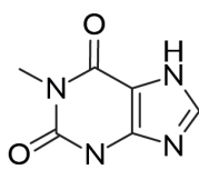
3. Theophylline
