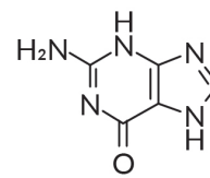
5. Guanine
